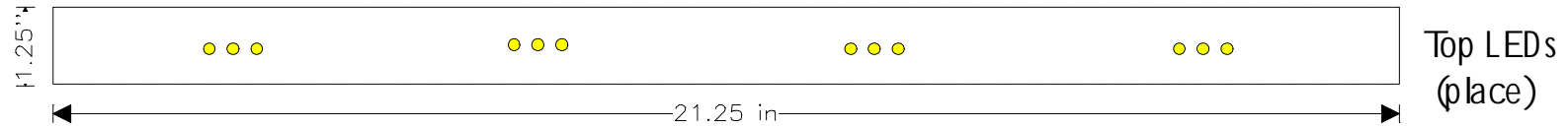
(Top View)
